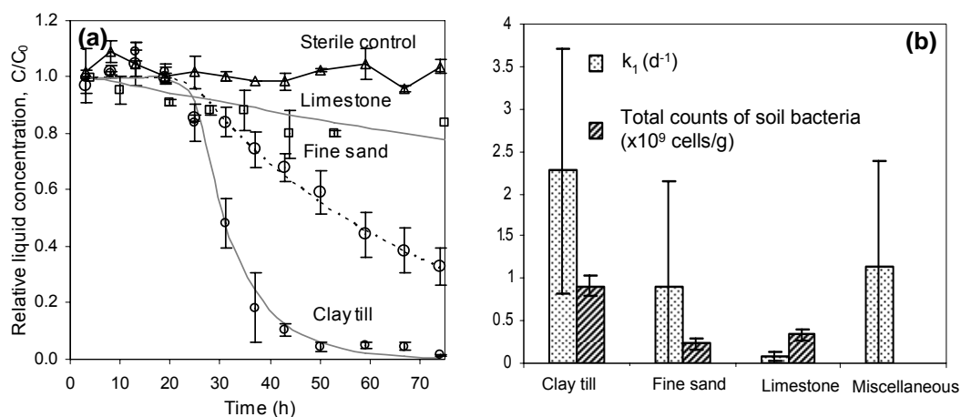
Figure 9 (a) Examples of benzene degradation curves from slurry reactor experiments; and (b) soil class averages of first-order rate constants ( k_1 ). Error bars represent the standard deviation (Paper I).
